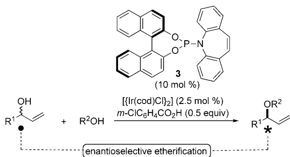
Scheme 1. Direct, enantioselective substitution of unactivated, branched allylic alcohols.
