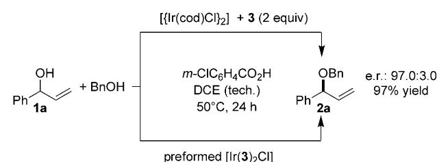
Scheme 2. Substitution reactions in technical-grade solvent with catalyst prepared in situ (top) and with preformed and purified catalyst [\text{Ir}(\mathbf{3})_2\text{Cl}] (bottom).
