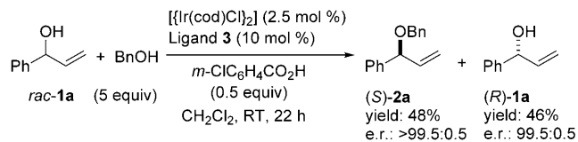
Scheme 3. Kinetic resolution at room temperature.
