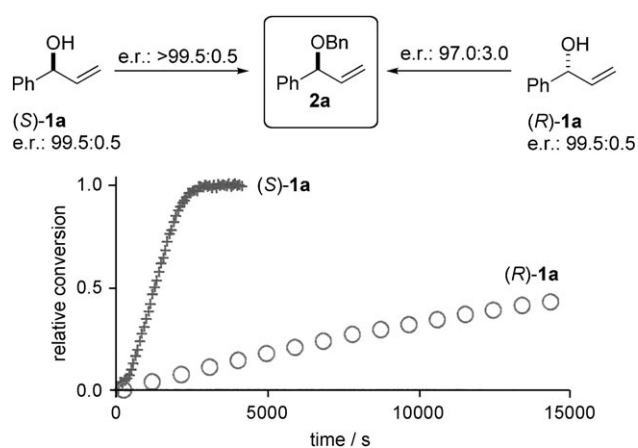
Figure 1. Profile for the allylic etherification for both substrate enantiomers, (S)-1a (+) and (R)-1a (○), monitored by ^1\text{H} NMR spectroscopy at 52°C. Full conversion of (R)-1a was observed after 1 day. [10]
